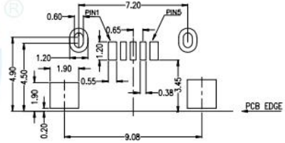
RECOMMENDED P.C.B. LAYOUT TOLERANCE UNSPECIFIED ±0.05mm
