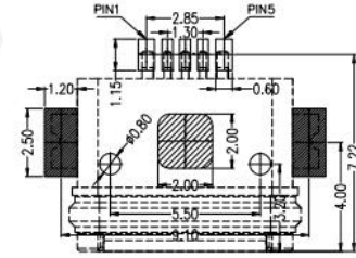
RECOMMENDED P.C.B. LAYOUT TOLERANCE UNSPECIFIED ±0.05mm
