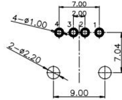
RECOMMENDED PCB LAYOUT(TOP VIEW)
