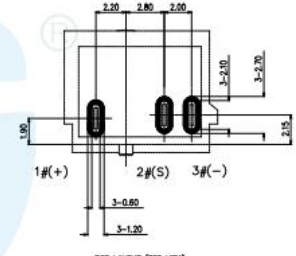
POB LAYOUT (TOP VIEW) TOLERANCE: ±0.05
