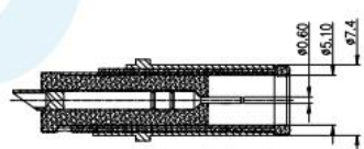
MATING PLUG: OD Ø7.4 ; ID Ø0.6 Tolerance:±0.05
