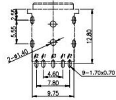
RECOMMENDED P.C.B LAYOUT TOP VIEW (TOLERANCE:±0.05)
