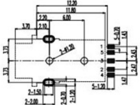
PCB LAYOUT (TOP VIEW) TOLERANCE: ±0.05
