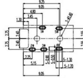
PCB LAYOUT (TOP VIEW) TOLERANCE: ±0.05
