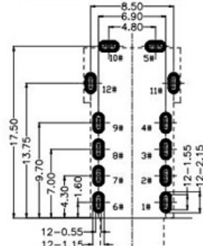
RECOMMEND PCB LAYOUT TOLERANCE:±0.05
