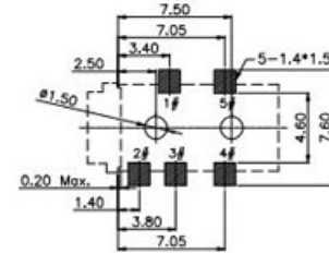
RECOMMENDED P.C.B LAYOUT TOP VIEW (TOLRANCE:±0.05)
