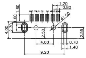
RECOMMENDED P.C.B LAYOUT TOP VIEW (TOLRANCE:±0.05)
