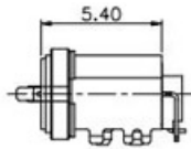
TYPE-C 16P 5.4L
