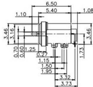
TYPE-C 16P 5.4L
