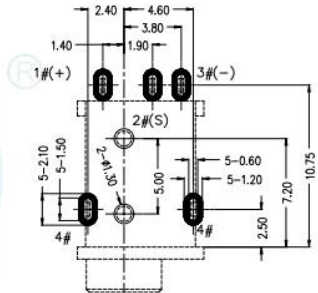
PCB LAYOUT (TOP VIEW) TOLERANCE: ±0.05
